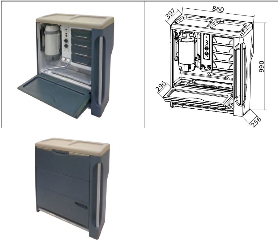
Type 05.3070.00.00 NEOPLAN
